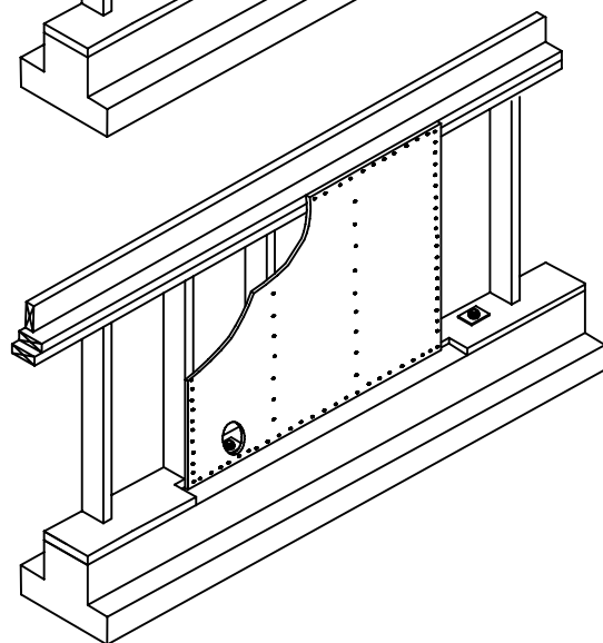
Sill Connection - Four panel flush cut
