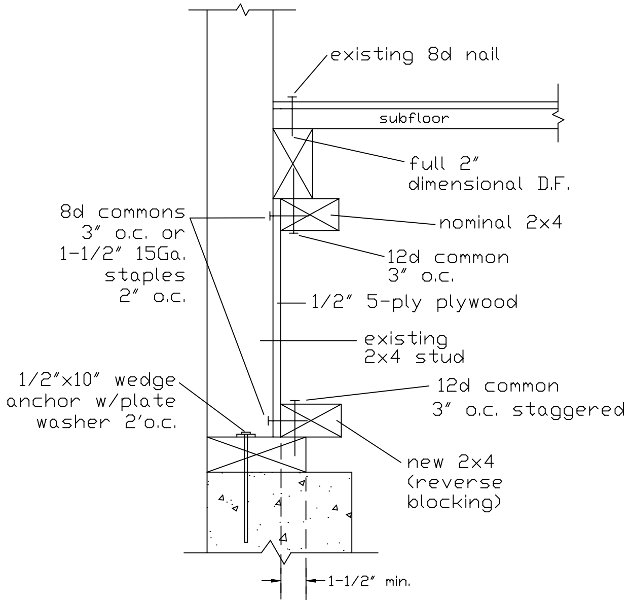
Detail for balloon framing when end floor joist is parallel to foundation. And detail for reverse blocking method on mudsill.
