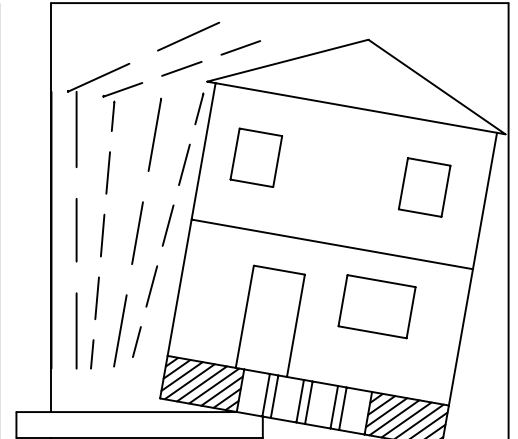
HOUSE AND CRIPPLEWALL FALL OFF FOUNDATION
