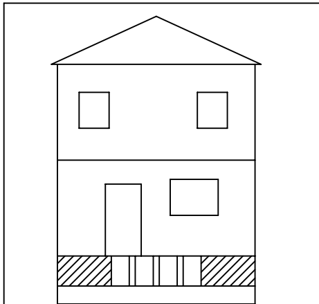
CRIPPLEWALL BRACED WITH PLYWOOD
