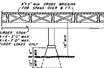
INTERIOR PIER FTG.
