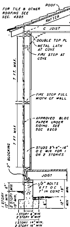
TYPICAL WALL SECTION
