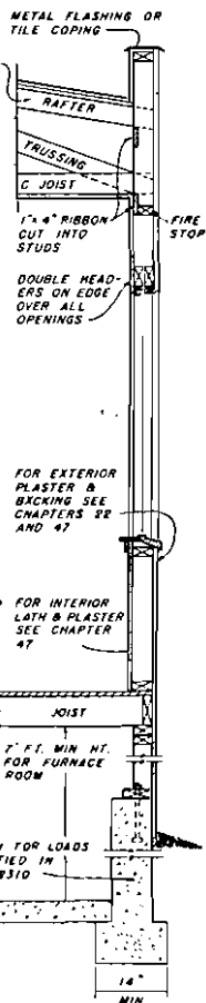
RETAINING WALL &amp; BALLOON FRAMING
