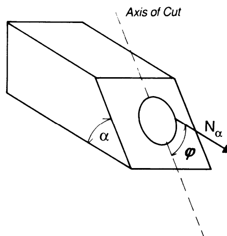
Figure 12I Sloping End Cut with Load at an Angle \phi to Axis of Cut
