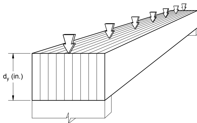
Figure 5B Depth, d_y , for Flat Use Factor
