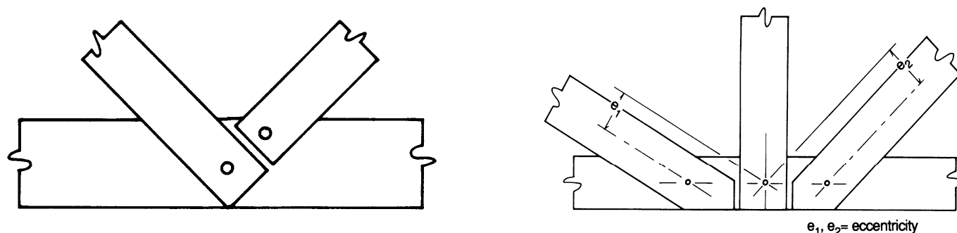
Figure 10A Eccentric Connections
