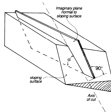
Figure 12E Axis of Cut for Asymmetrical Sloping End Cut
