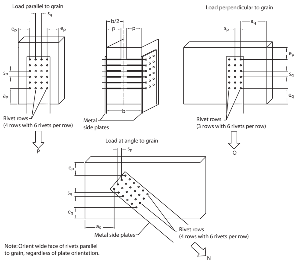
Figure 13A End and Edge Distance Requirements for Timber Rivet Joints
