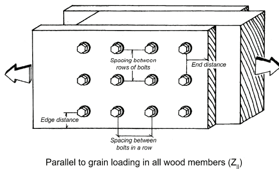
Figure 11G Bolted Connection Geometry
