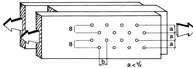
Figure 10B Group Action for Staggered Fasteners
