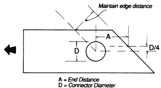
Figure 12K End Distance for Members with Sloping End Cut
