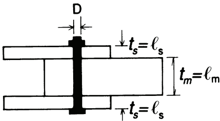
Figure 11C Double Shear Bolted Connections
