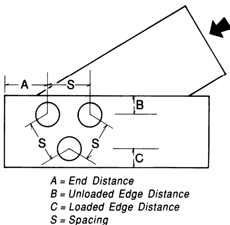
Figure 12J Connection Geometry for Split Rings and Shear Plates
