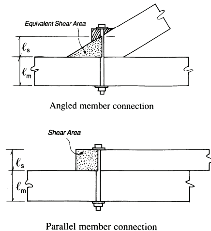
Figure 11E Shear Area for Bolted Connections
