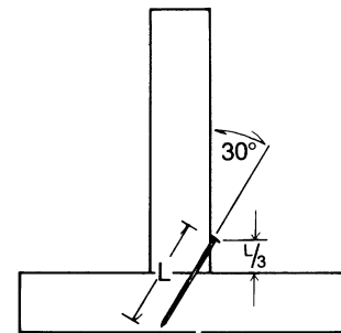
Figure 11A Toe-Nail Connection
