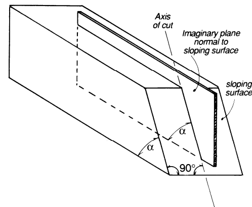
Figure 12E Axis of Cut for Asymmetrical Sloping End Cut
