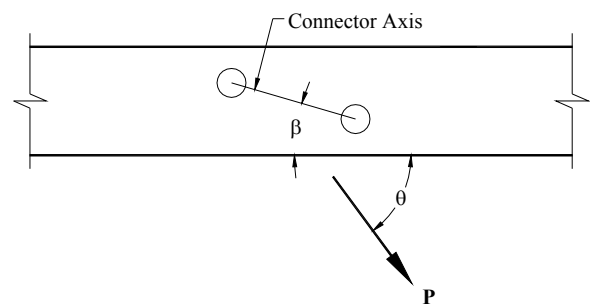
Figure 12L Connector Axis and Load Angle
